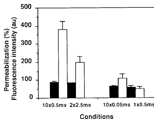
FIGURE 4 Effect of pulse duration and number of pulses at a given electroporation time. Cells were pulsed at 1 kV/cm intensity at various pulse durations and numbers of pulses whose product was kept constant and equal to 0.5 or 5 ms (i.e., 10 pulses lasting 0.5 ms and 2 pulses lasting 2.5 ms or 10 pulses lasting 50 \mu s and 1 pulse lasting 0.5 ms) at a 1 Hz frequency. The percentage of permeabilized cells to propidium iodide (black histogram) and the associated fluorescence intensity (white histogram) are plotted as a function of these different conditions.
